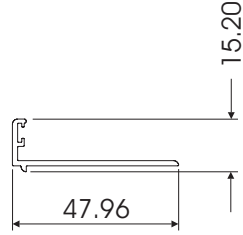
CLIP44 ASTRAGAL WITH WOOLPILE CL206
