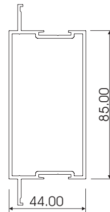
CLIP44 R4-SPECIAL MID RAIL 85mm CL18A
