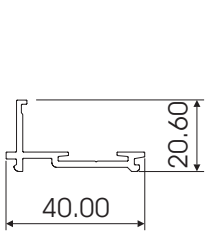
CLIP44 R4 FILLER ADAPTOR CL19A
