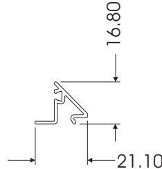
CLIP44 ANGLED GLAZING BEAD CL225
