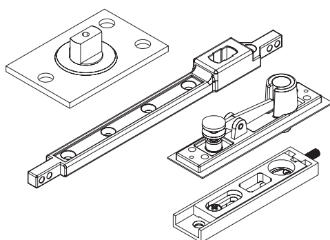
TOP CENTRE STRAP + PIVOT
