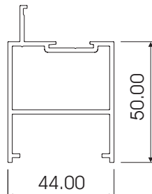
CLIP44 R7 HEAD/ SILL RAIL 50mm CL22A
