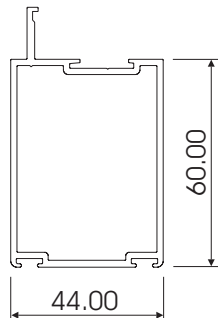
CLIP44 R11W D/STILE 60mm W/PILE CL221
