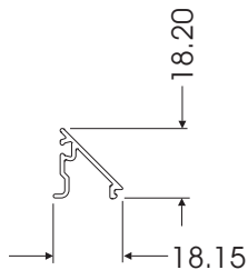
NEW CLIP44 ANGLED GLAZING BEAD CL13A
