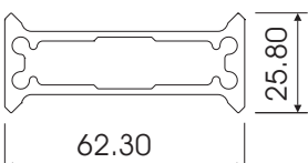
CLIP44 BOX SPIGOT 4 X S/PORT W55456
