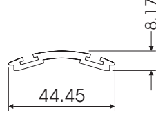
CLIP44 SILL ADAPTOR CL104
