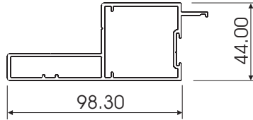
MAGLOCK DOUBLE DOOR STILE OPENING DOOR CL95
