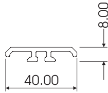
COLONIAL BAR CL208
