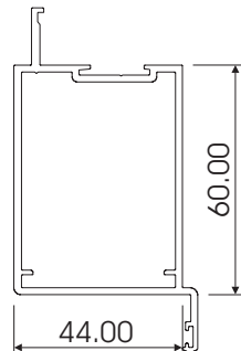
CLIP44 R11SP D/STILE 60mm CL227
